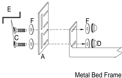
Attachment of Modi Plate to Metal Bed Frame
