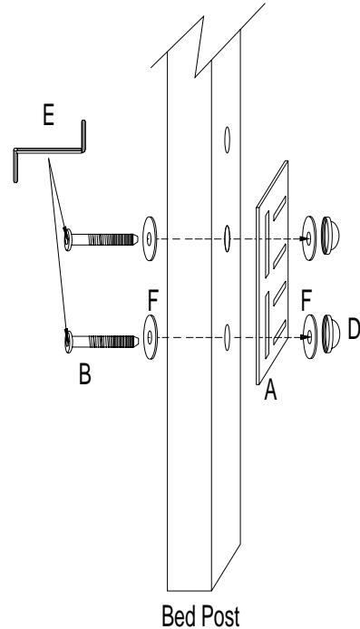
Attachment of Modi Plate to bed/ Headboard
